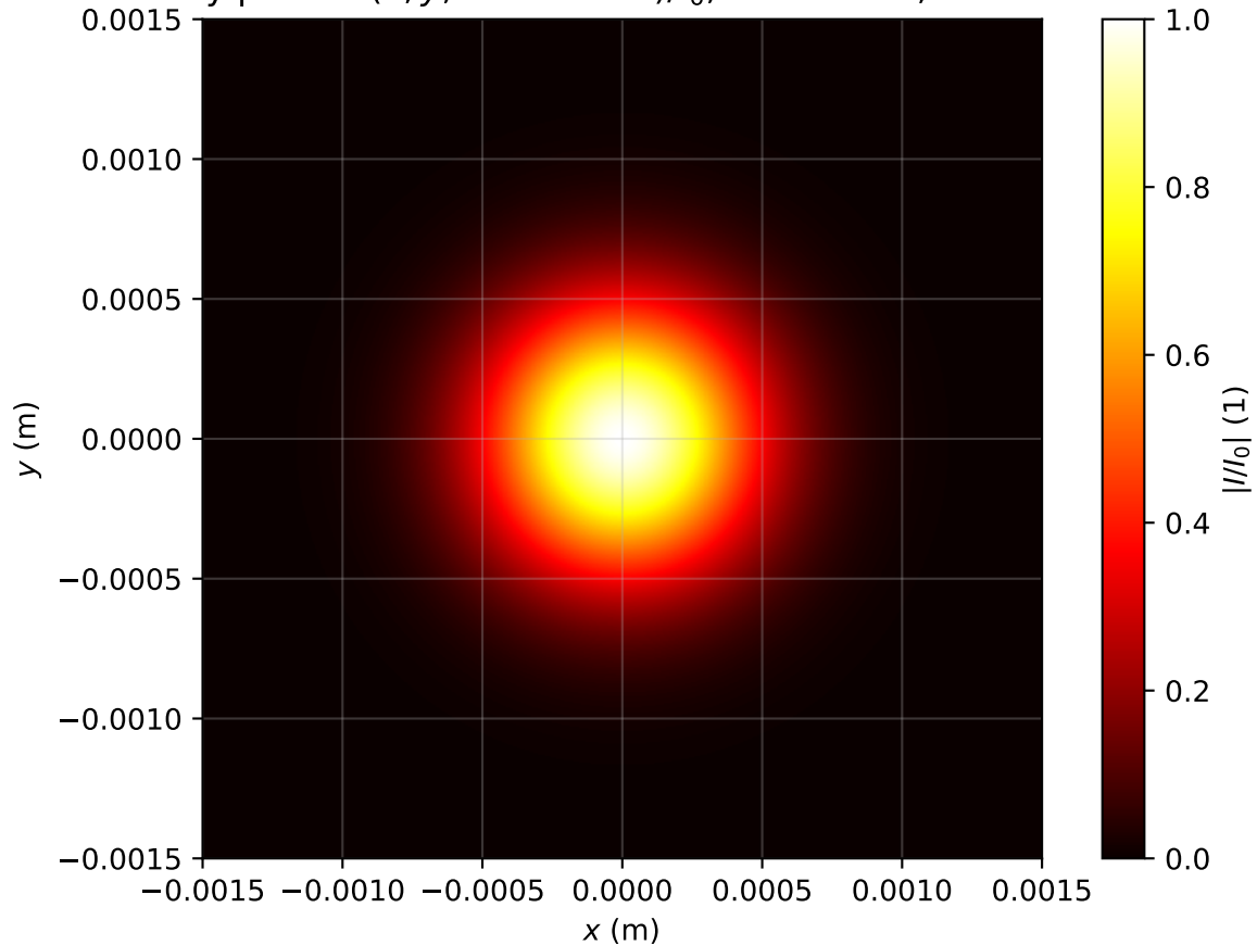
Intensity profile I(x, y, z = 0.000\text{m})/I_0 , \text{Pin}=0.7\text{Pcr} , artificial time
